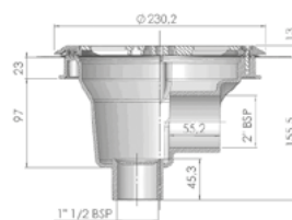
B-B Section
